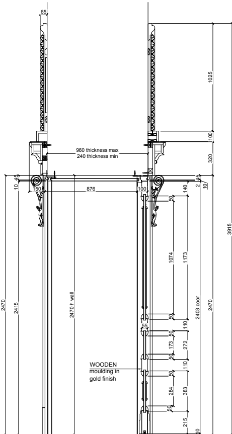
SECTION "D" sc.1:10
