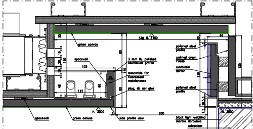
DETAIL 03
