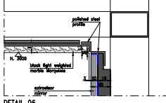
DETAIL 06
