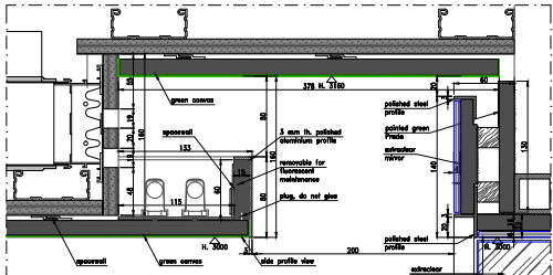
DETAIL 02
