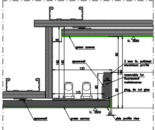
DETAIL 05
